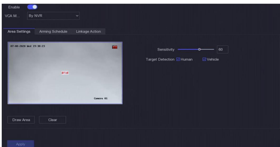
Figure 5-10 Motion Detection
