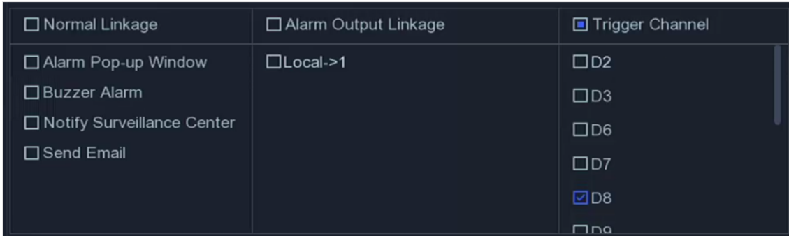
Figure 5-12 Linkage Actions
