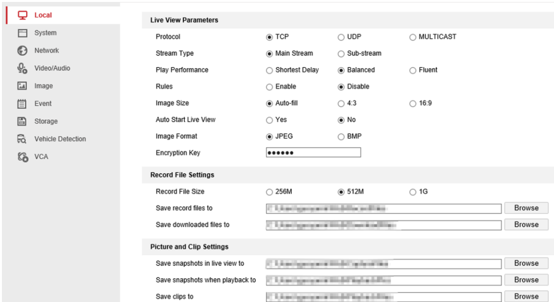
Figure 9-4 Configuration
