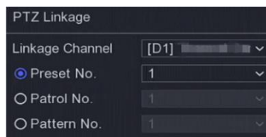
Figure 6-30 PTZ Linkage
