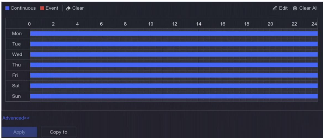
Figure 6-31 Recording Schedule
