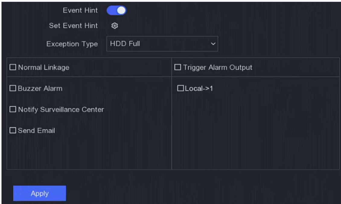
Figure 6-23 Exceptions
