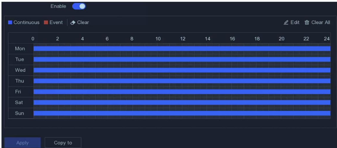
Figure 5-14 Recording Schedule
