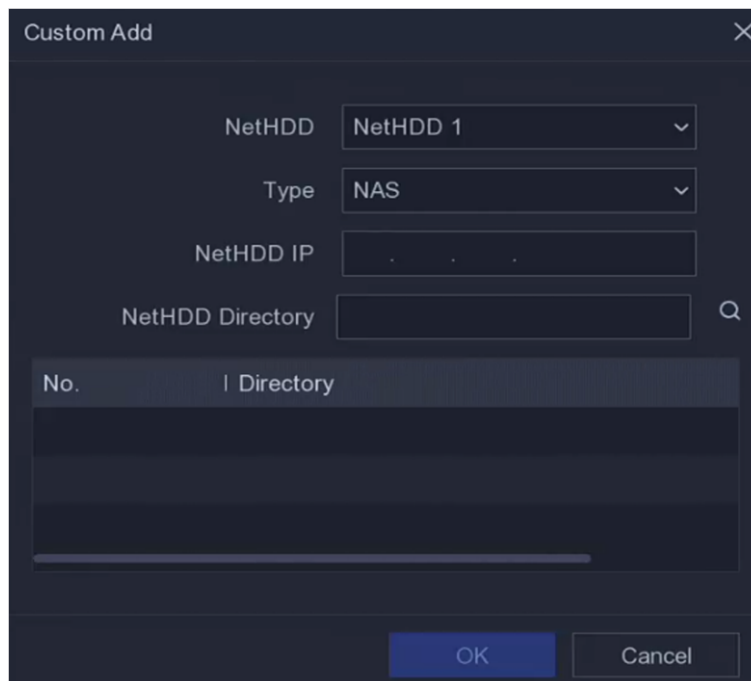
Figure 5-13 Add NetHDD
