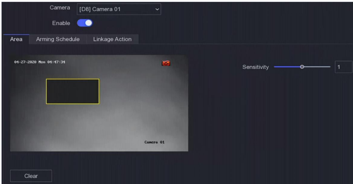
Figure 6-18 Video Tampering
